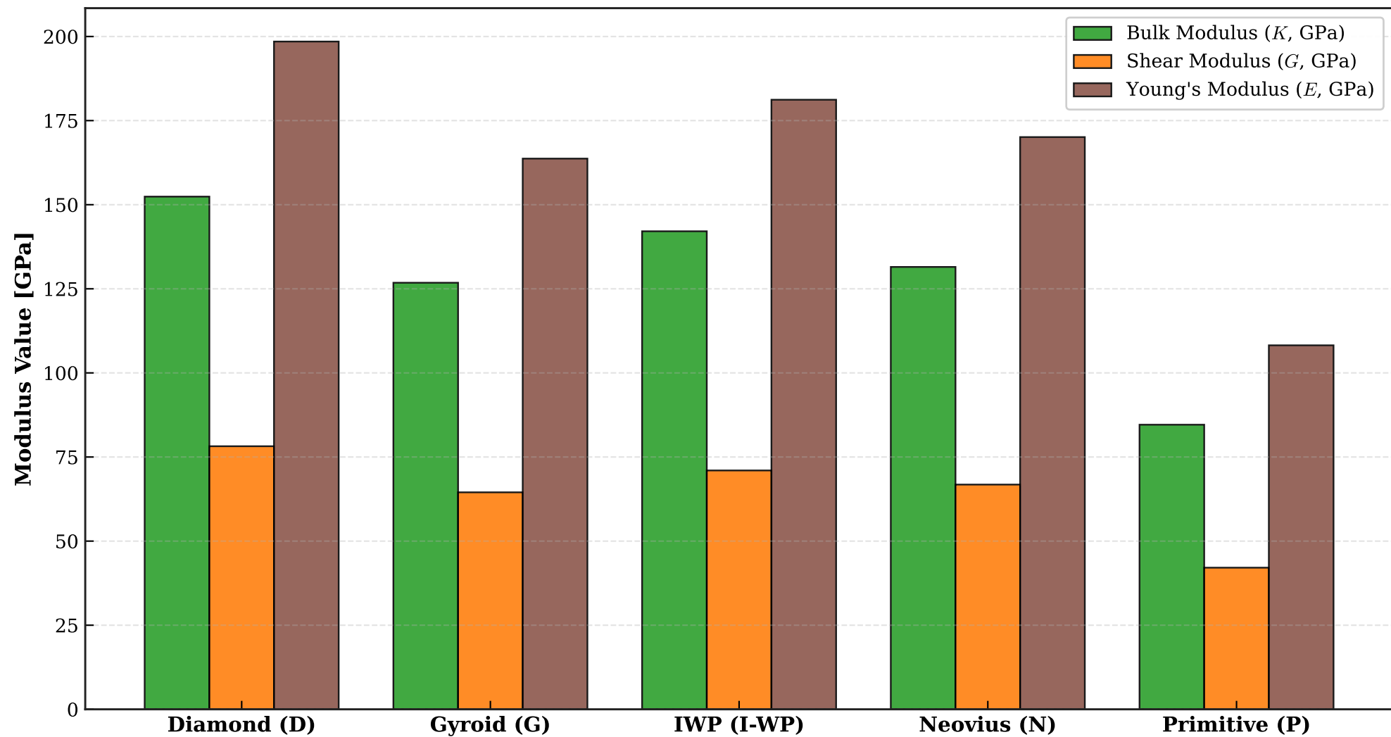
Elastic Mechanical Moduli Across 5 Graphene TPMS Topologies
